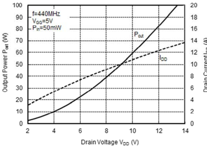
OUTPUT POWER versus DRAIN VOLTAGE
