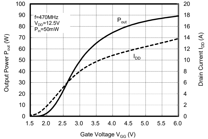
OUTPUT POWER, DRAIN CURRENT versus GATE VOLTAGE
