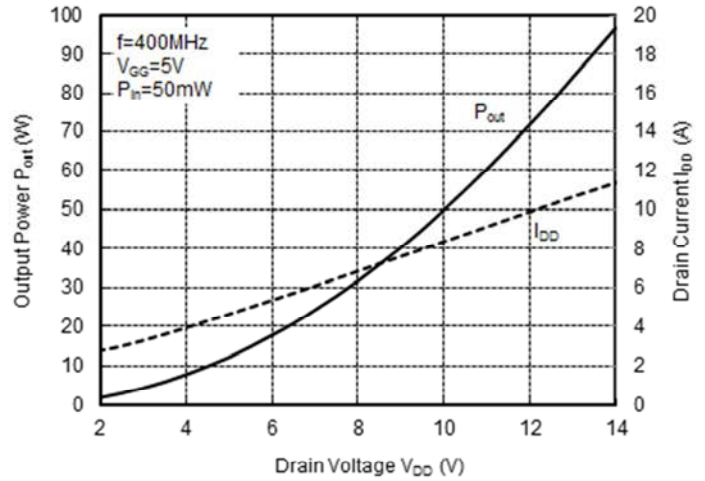
OUTPUT POWER, DRAIN CURRENT versus DRAIN VOLTAGE
